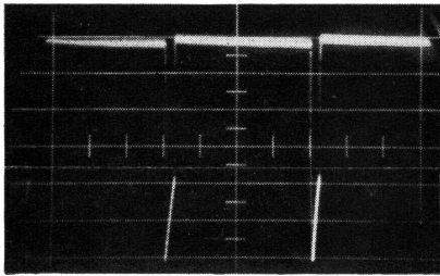
Fig. 7. VERTICAL BLKG at G-1 of CRT, 75V P.P.
