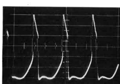
Fig. 11. HORIZONTAL DISCHARGE GRID PULSE G-1 of (V-9B) Pin 2, 60V P.P.
