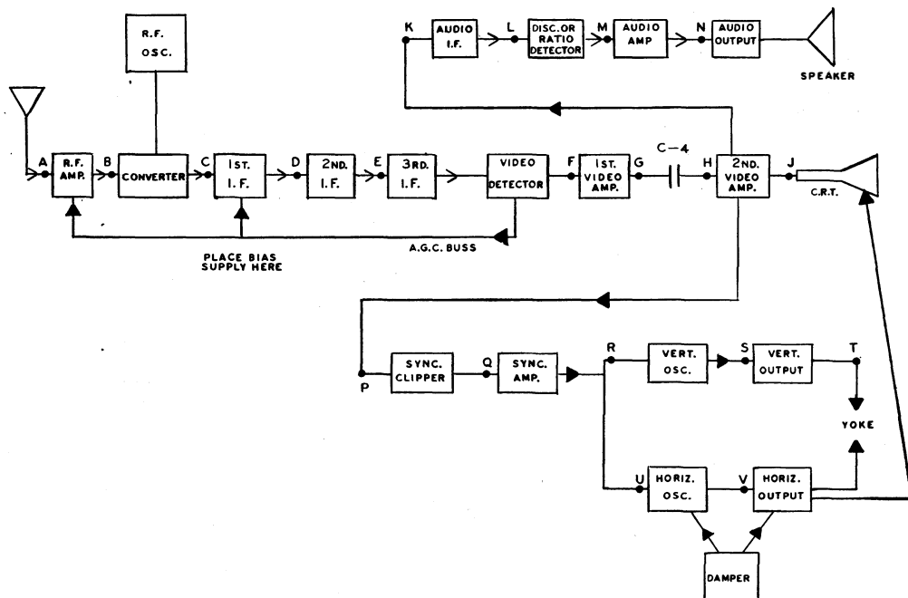
Figure 4—Block diagram of typical TV receiver
