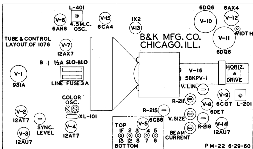
Figure 2 Layout of tubes and controls of the Analyst
