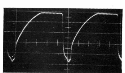
Fig. 12. HORIZONTAL SAW at G-1 of horizontal amp (V-10), 150V P.P.
