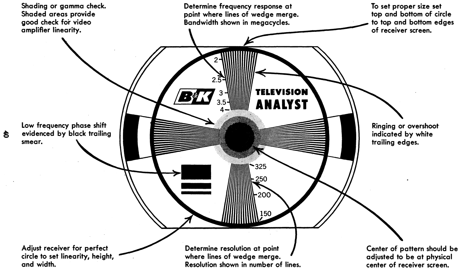
Figure 25—Test Pattern
